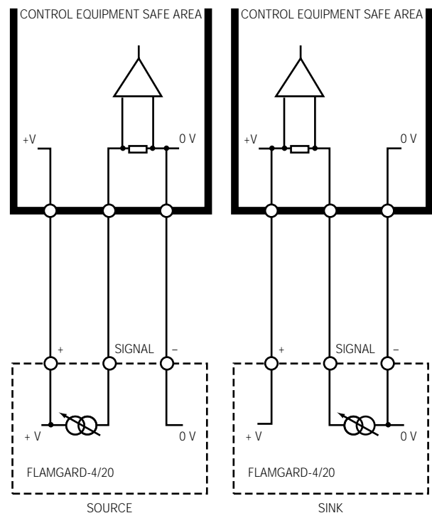
Diagram 3: Electrical connections
